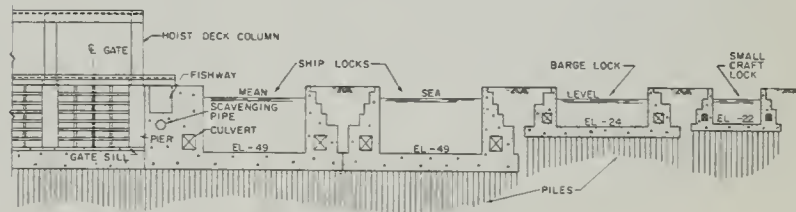
TYPICAL SECTION OF FISHWAY AND LOCKS
